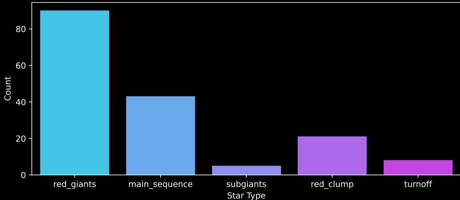
APOGEE DR17 Field: [206+21] Count plot of Star Type
