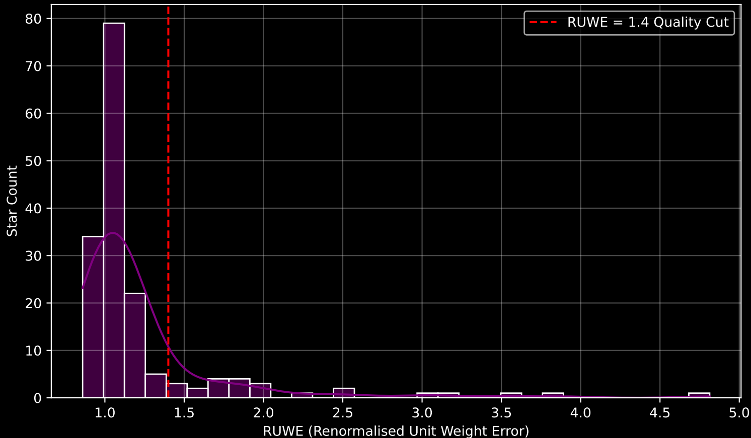
GAPOGEE DR17 Field [206+21] RUWE Distribution (n= 164)
