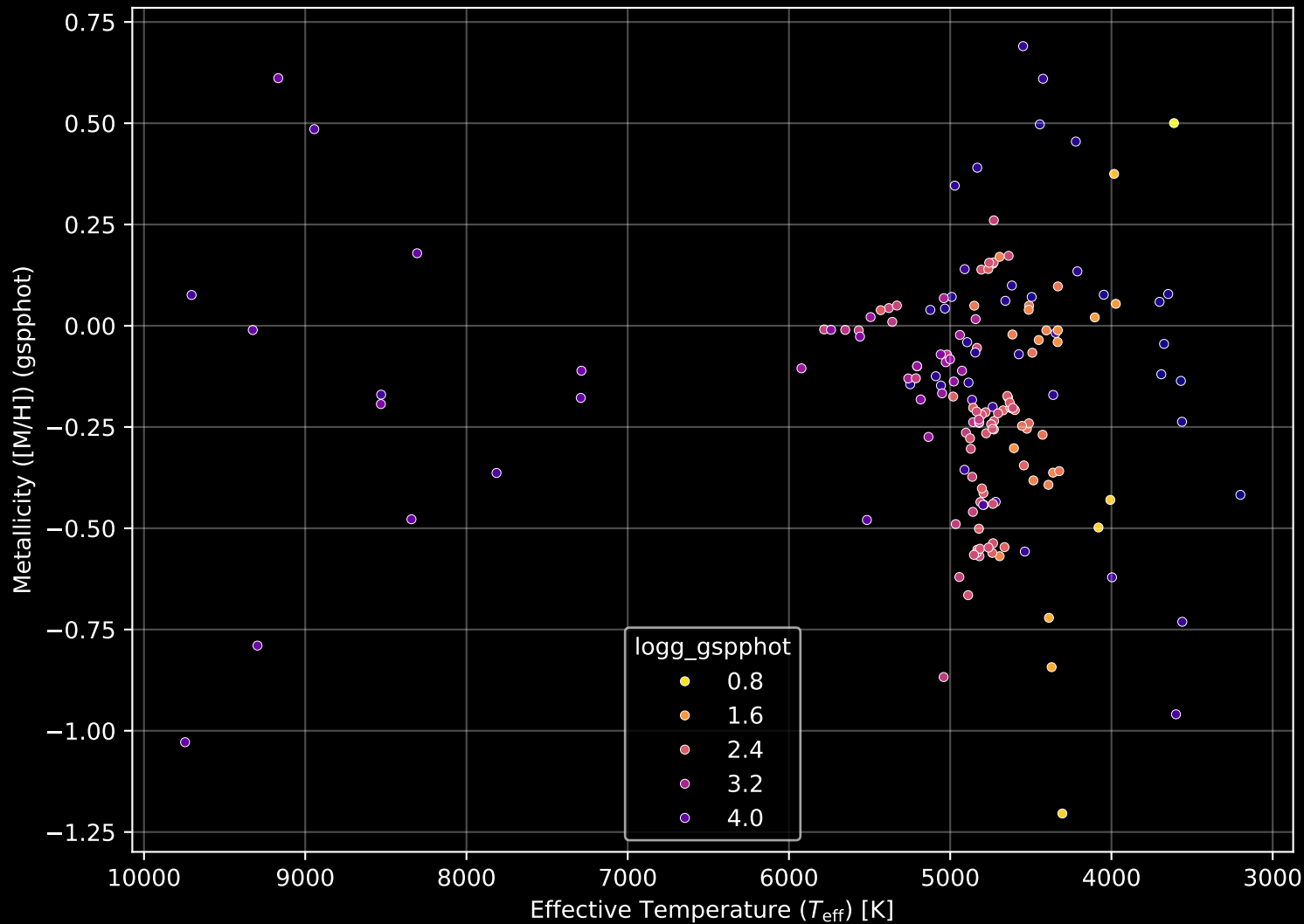
APOGEE DR17 Field: [206+21] Stellar Population Parameters (n= 167)
