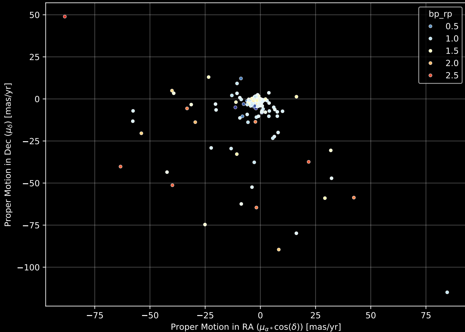
APOGEE DR17 Field: [206+21] Proper Motion Diagram (n= 167)
