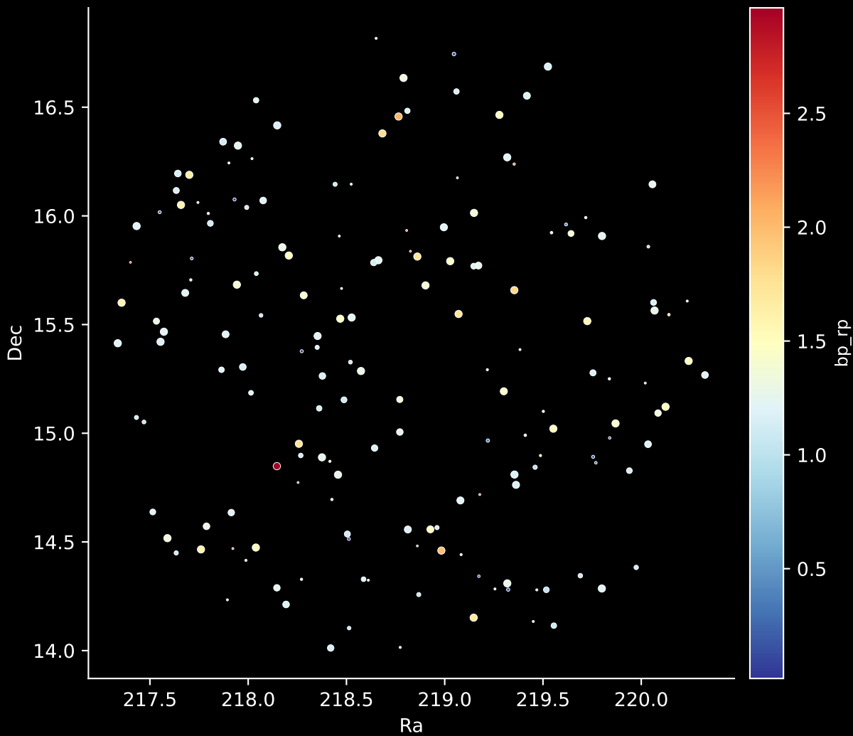
APOGEE DR17 Field: [206+21] Stars: 167
