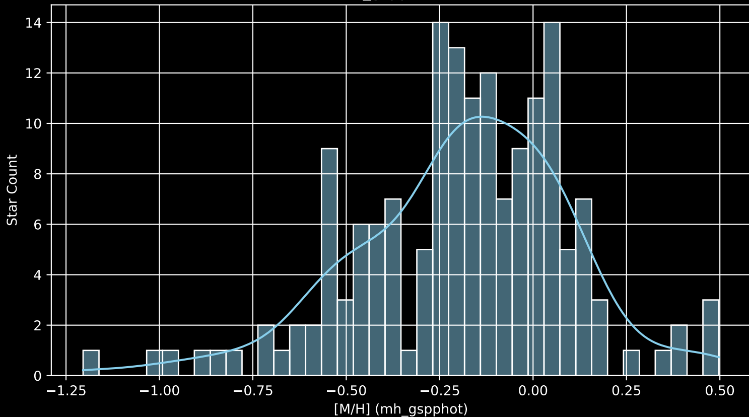
APOGEE DR17 Field: [206+21 [M/H] (mh_gspphot) (n= 163)
