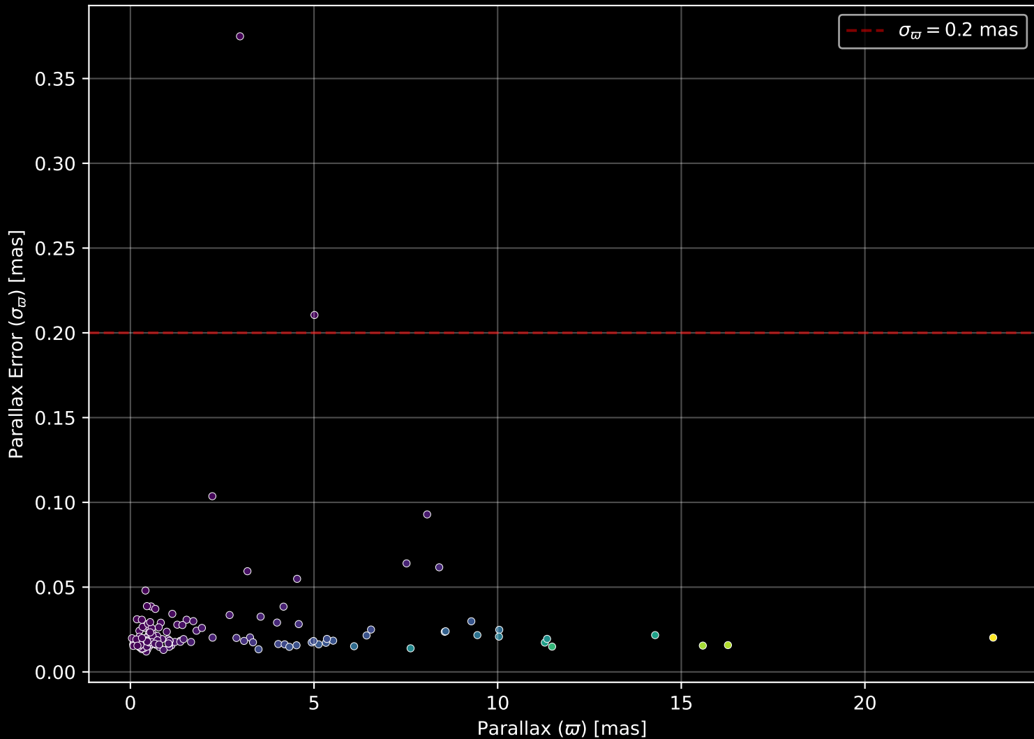
APOGEE DR17 Field: [206+21] Parallax Quality (n= 167)
